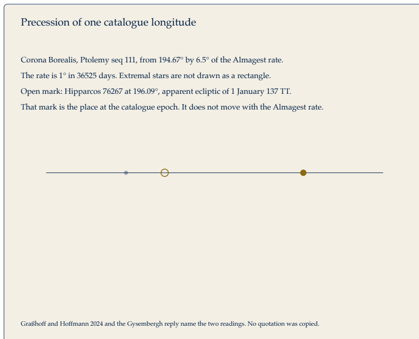
Figure 6 Catalogue longitude of Corona Borealis seq 111, carried 6.5^\circ by the Almagest rate. The open mark is Hipparcos 76267 at the catalogue epoch.
