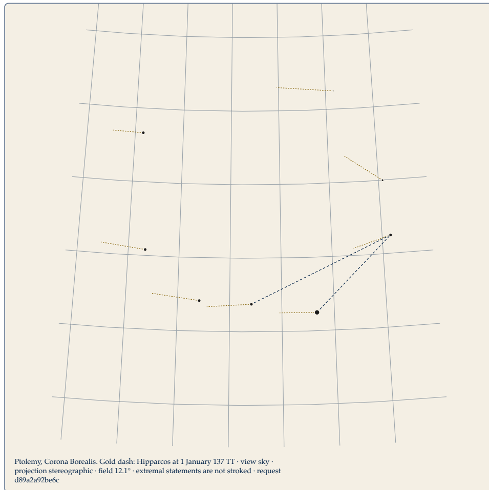
Figure 1 Corona Borealis in the Ptolemy catalogue. The dark dashed stroke is a membership line. The short gold dashes run to the Hipparcos places at 1 January 137 TT. An extremal path in the same request is not drawn.
