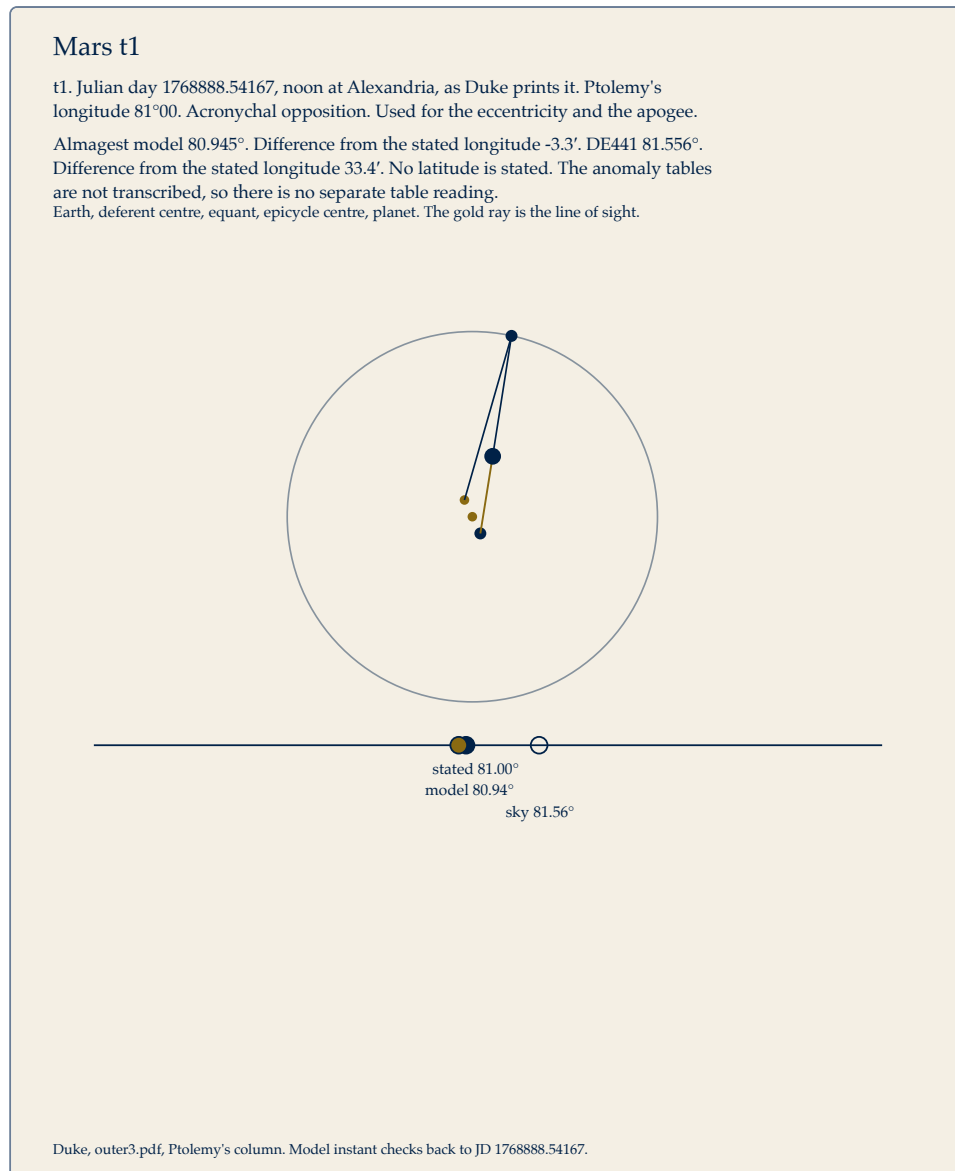
Figure 9 Mars t1. Stated longitude 81;00. The model is 3.3 arcminutes west of it. DE441 is 33.4 arcminutes east of it.
