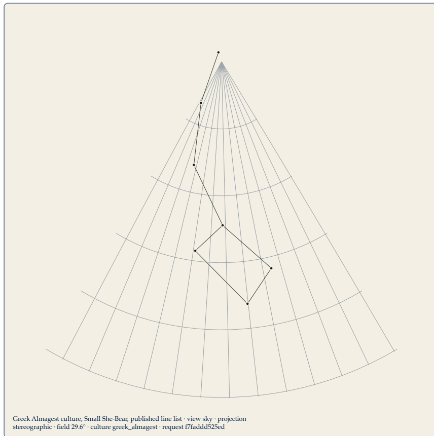
Figure 2 The Small She-Bear in the Greek Almagest sky culture. The line is the published Hipparchos sequence, drawn in equatorial coordinates.
