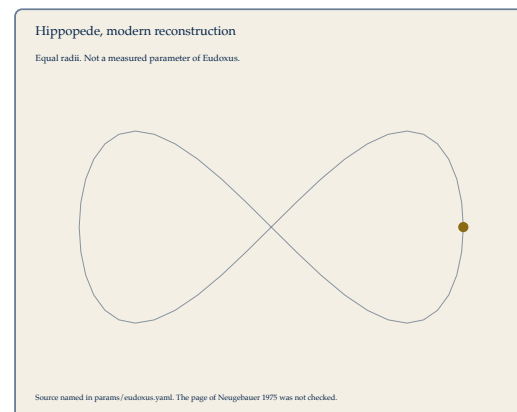
Figure 8 The hippopede with equal radii, labelled as a reconstruction.
