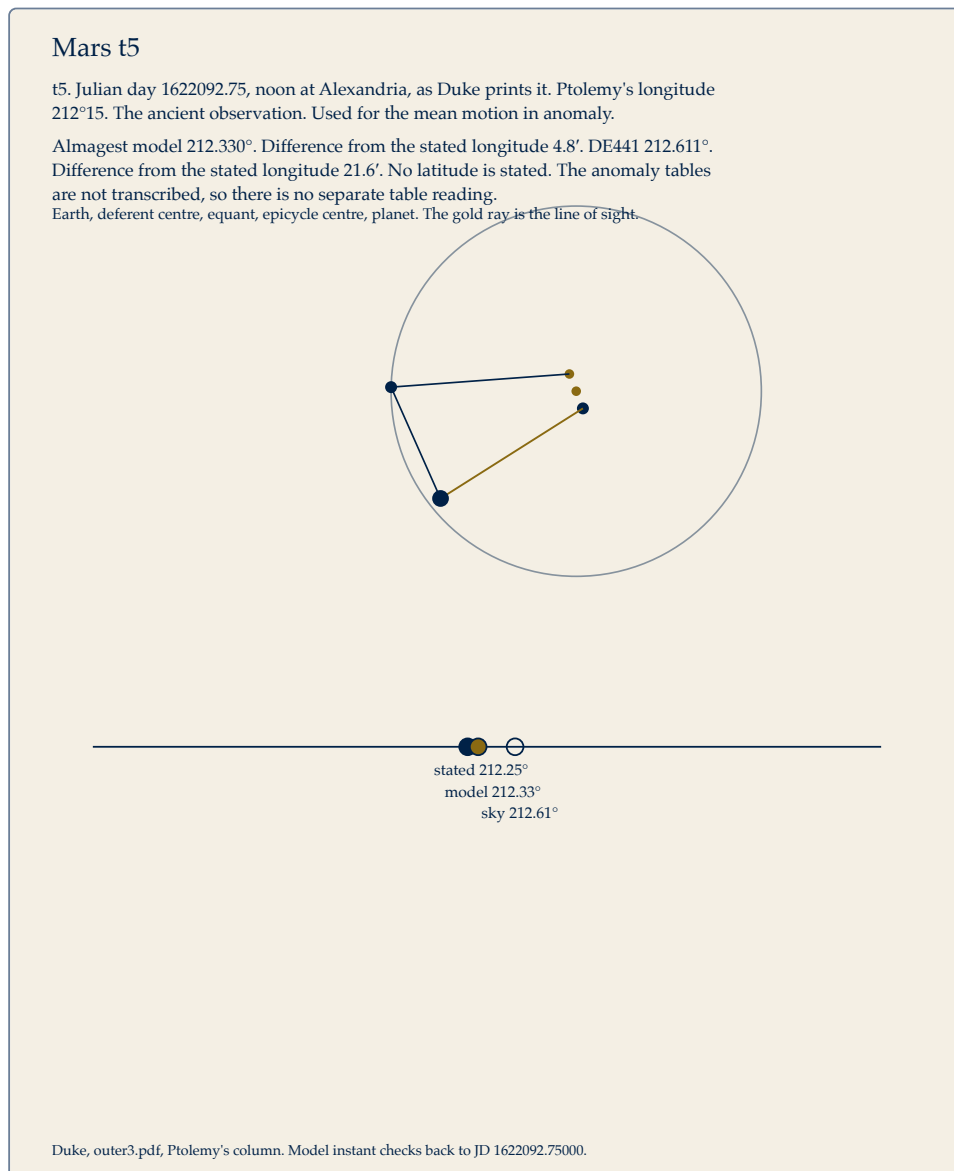
Figure 13 Mars t5. Stated longitude 212;15. The model is 4.8 arcminutes east of it. DE441 is 21.6 arcminutes east of it.
