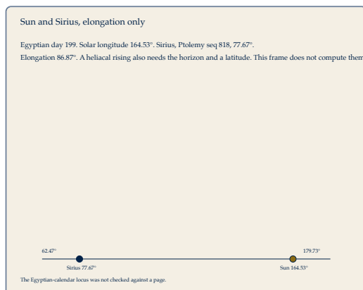
Figure 7 Solar elongation from the catalogue longitude of Sirius. The horizon is not part of the frame.
