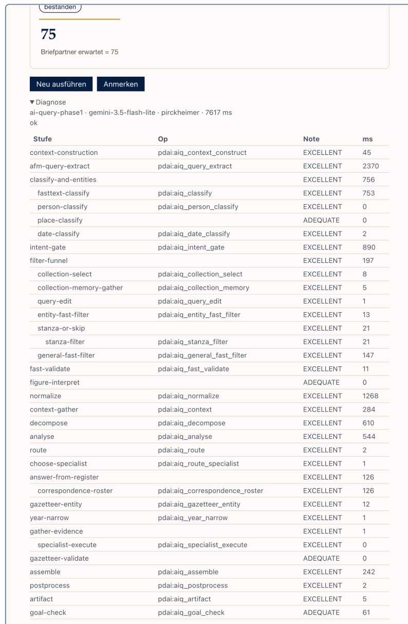
Figure 9 The fold Diagnose of the subtask ch02/subtask-count : origin line and trace. Each row is a stage, with its operation, its grade and its time.
